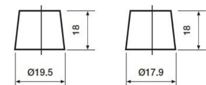
Positive Terminal
