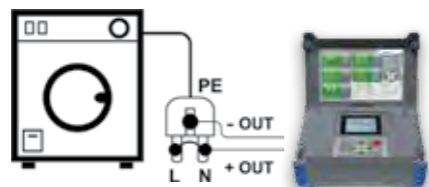
Measurement of household device, protection class I and class II
