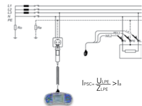
Circuit for measurement of fault loop impedance
