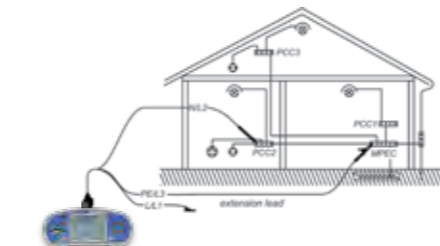
Test circuit for continuity R200 mA measurement
