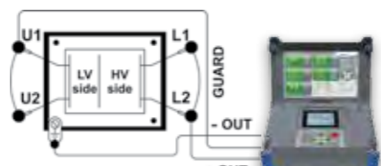
The simplest measurement of insulation resistance of transformer
