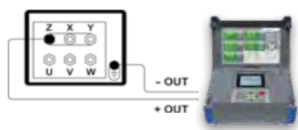
Measurement of insulation resistance of induction motor between all three phases against metal enclosure
